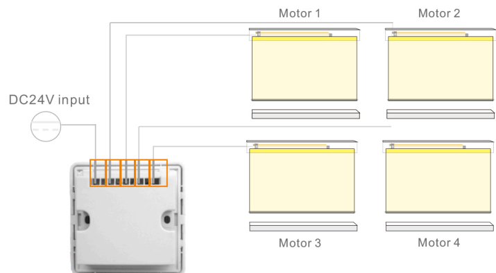
Wiring diagram
